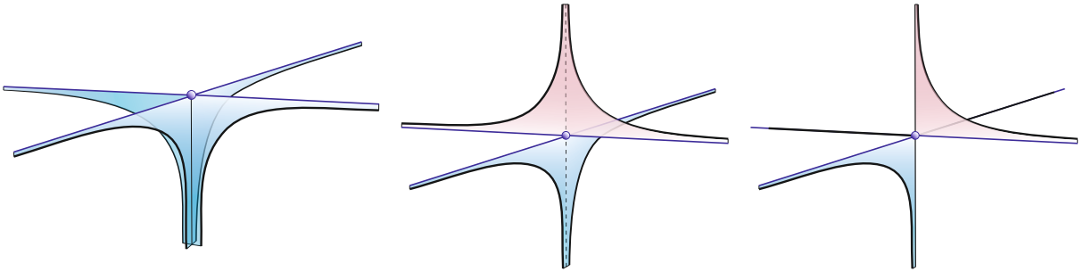
Figure. The “classic” and exotic Coulomb potentials
